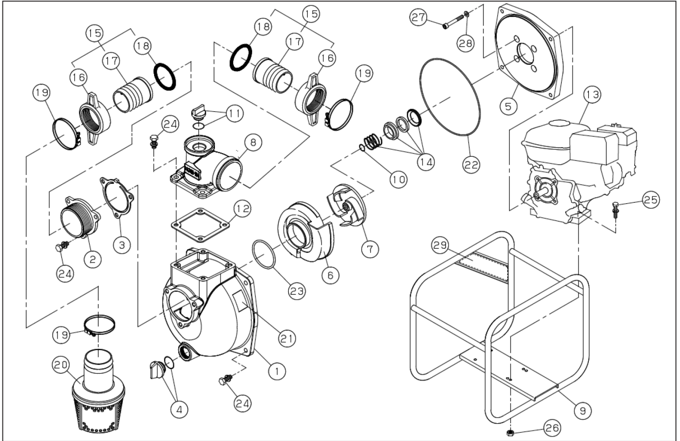
DWG No.012930409 MODEL : SEH-80JP FORM : SEH-80JP-BAB-1 (GP160)
