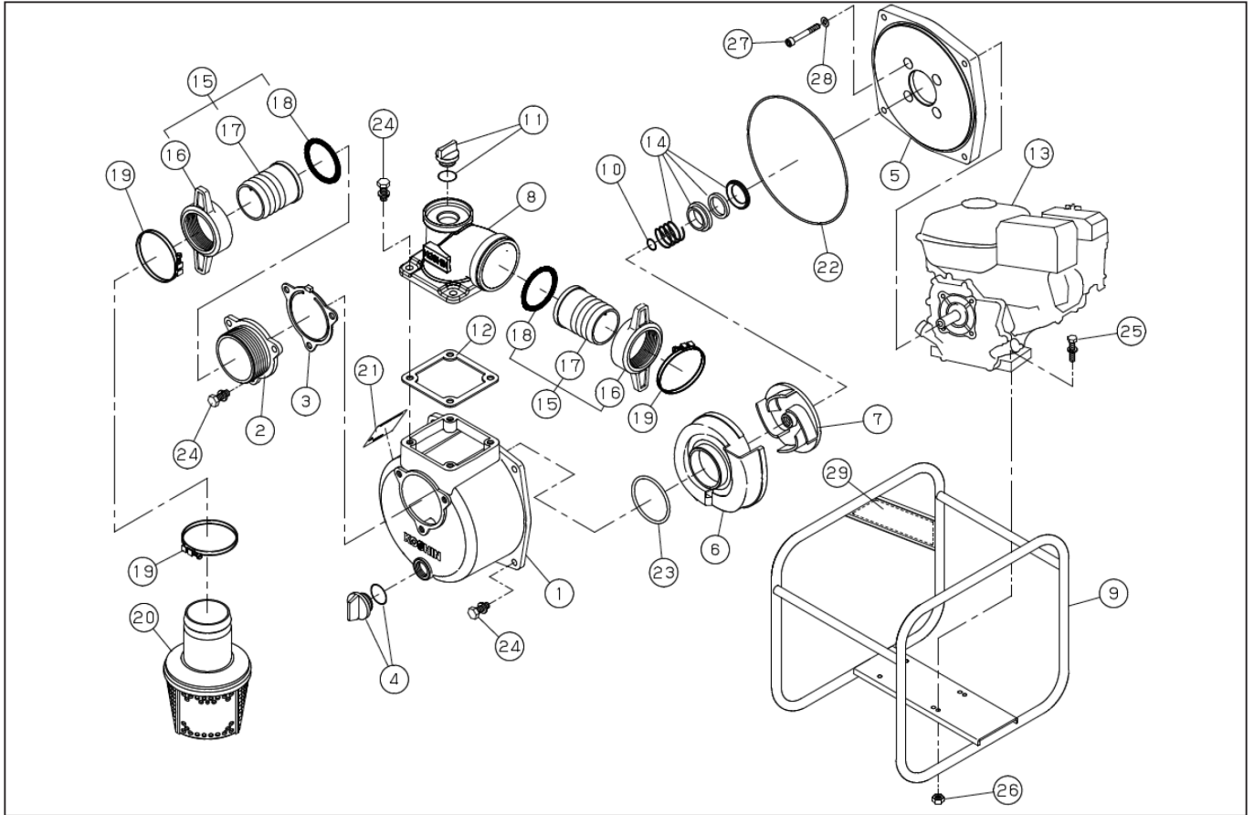
DWG No.012948807 MODEL : SEH-80P FORM : SEH-80P-BAC-1 (GP160)
