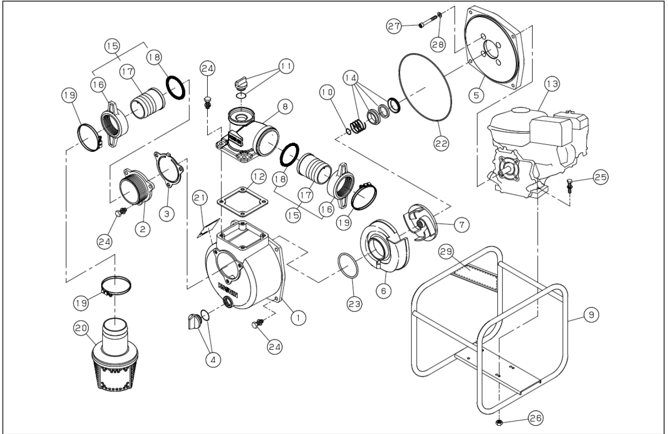
DWG No.012935609 MODEL : SEH-80X FORM : SEH-80X-BFQ-2 (GX160H2)
