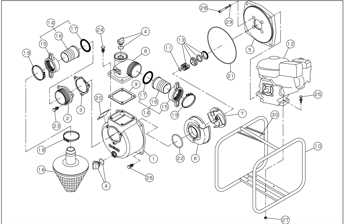
DWG No.013857401 MODELE:SEV-50E FORM:SEV-50E-BAB-0 (K210S)
