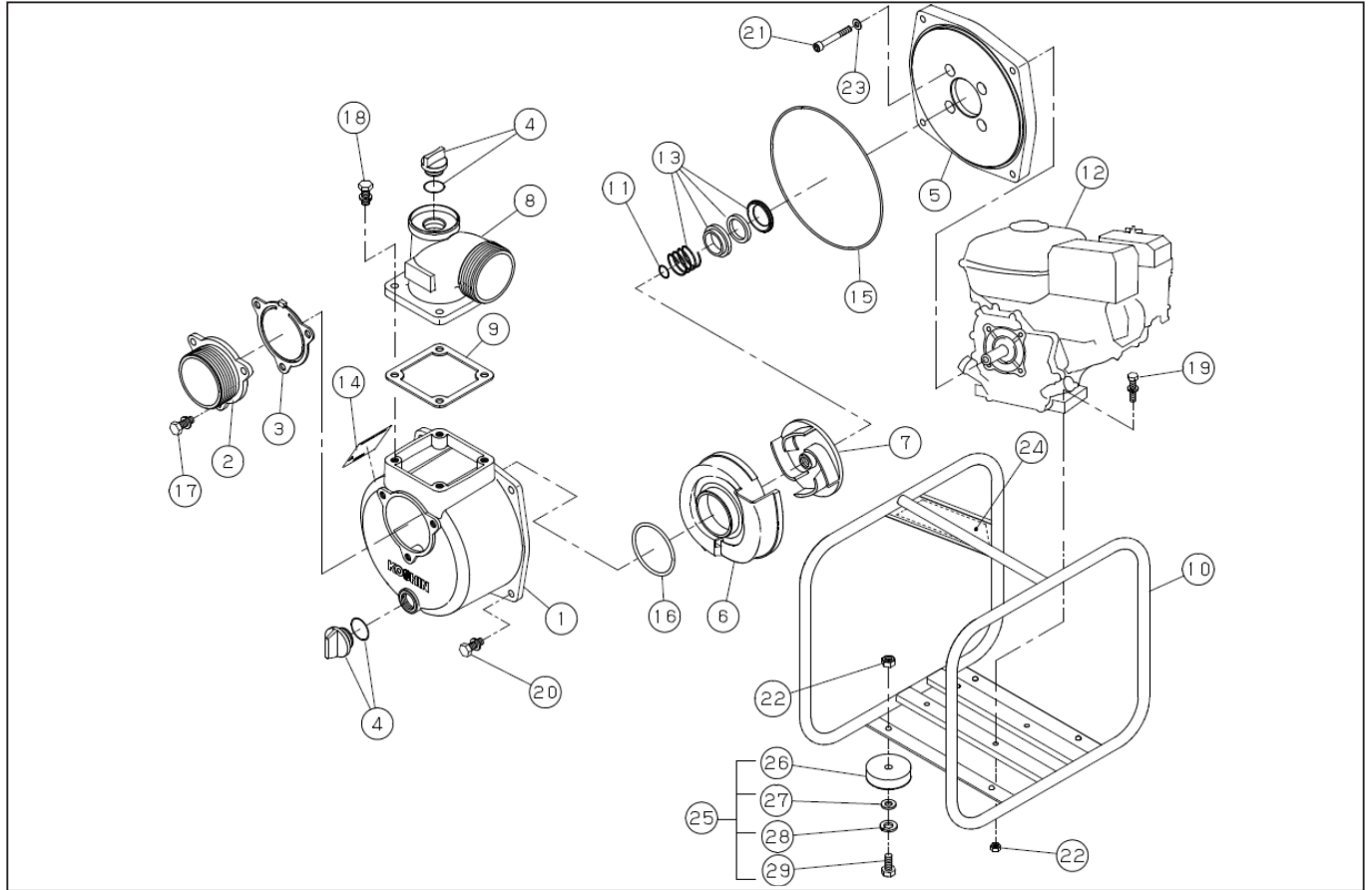
DWG No.013857801 MODELE:SEV-50E FORM : SEV-50E-BAC-0 (K210S)
