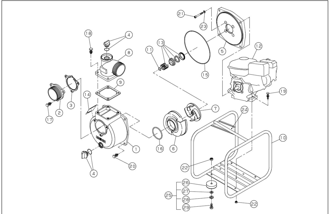
DWG No.012911412 MODEL : SEV-50X FORM : SEV-50X-BAH-3
