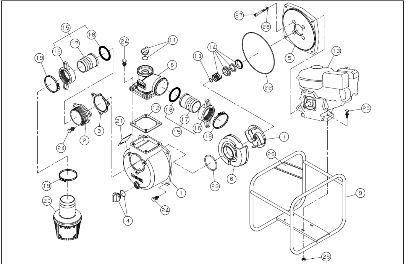
DWG No.012910226 MODEL : SEV-80X FORM : SEV-80X-BAC-9
