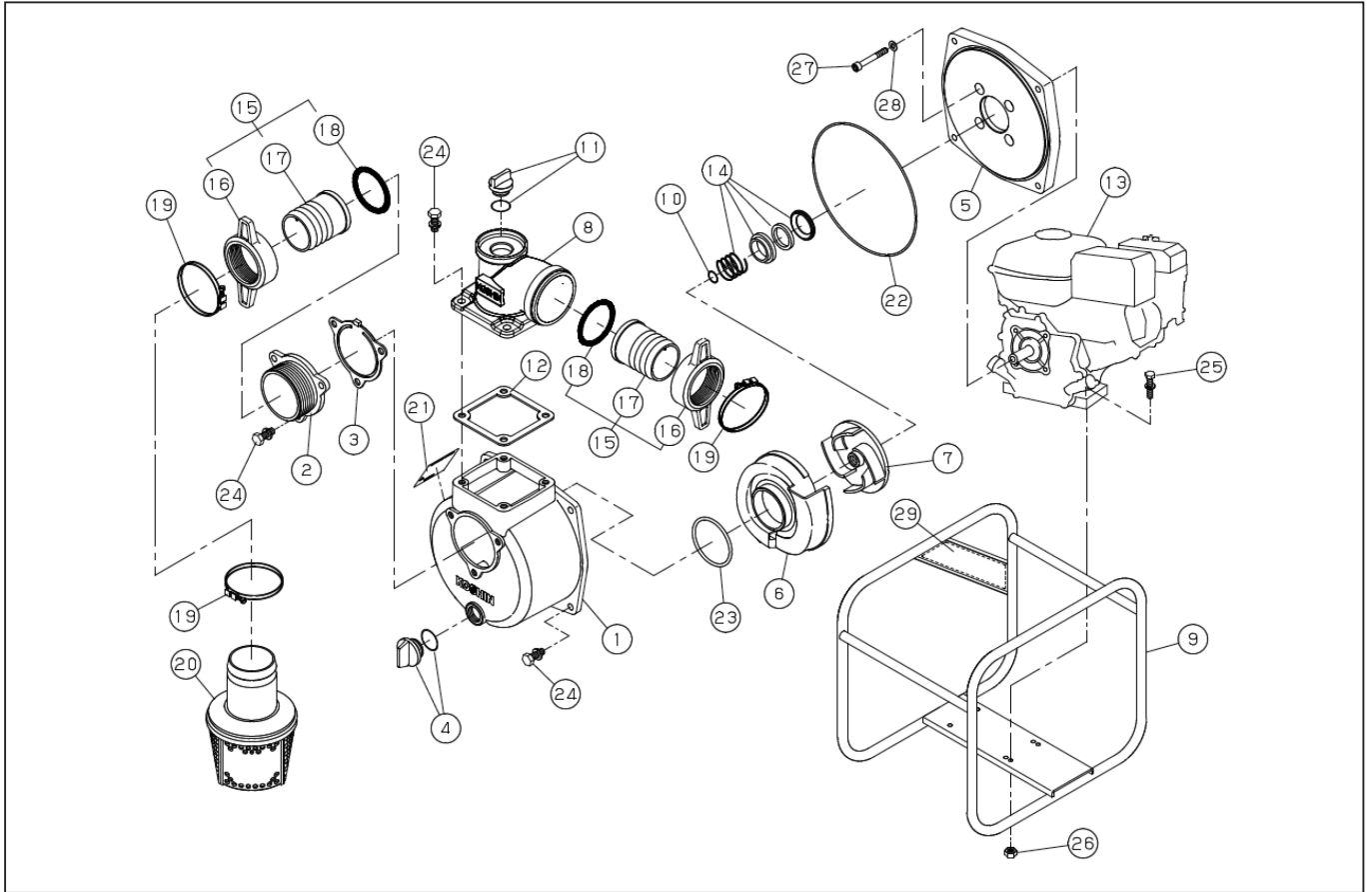
DWG No.012922414 MODEL : SEV-80X FORM SEV-80X-BAM-5
