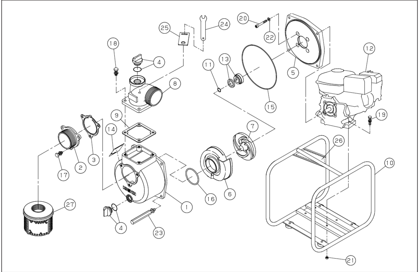
DWG No.012912713 MODELE : STV-50X FORM : STV-50X-BAB-2 (K180)
